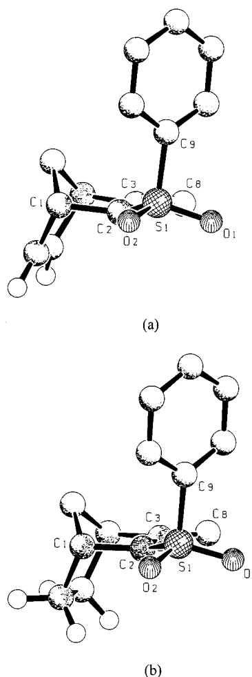
Figure 8. Calculated (HF/6-31+G*) structures of exo-3(-Li + ) (a) and exo-4(-Li + ) (b)
