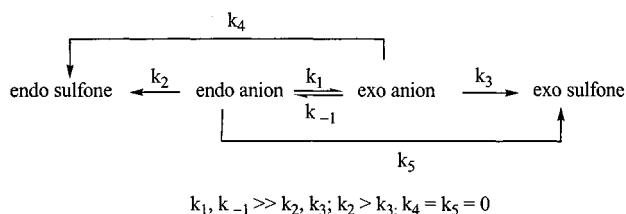
Scheme 8. Simplified kinetic scheme for the reaction of the endo and exo conformers of carbanions 3 and 4 with electrophiles
