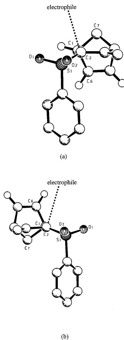
Figure 9. Modell for the trajectory of attack of electrophiles on the exo face of endo-3 (-Li + ) (a) and on the endo face of exo-3 (-Li + ) (b); the views are constructed from the calculated coordinates of endo-3 (-Li + ) and exo-3 (-Li + ) by picturing the trajectory manually
