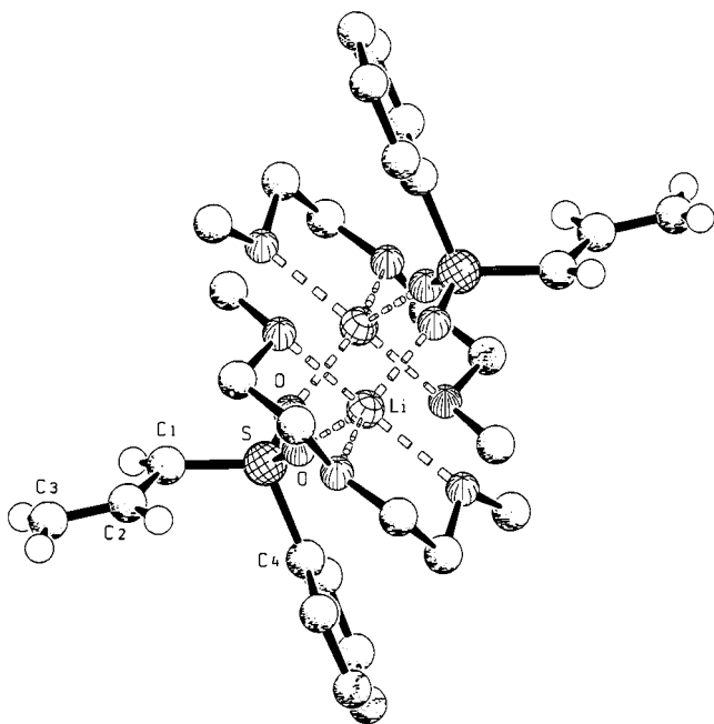
Figure 6. Crystal structure of 7/ ent -7·2diglyme; the view is constructed from the published coordinates; [16] selected bond lengths [Å]: S–C1 1.668(5), C1–C2 1.445(5), C2–C3 1.352(9)
