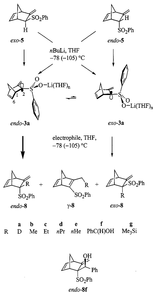
Scheme 5. Reaction of the lithioallyl sulfone 3 with electrophiles
