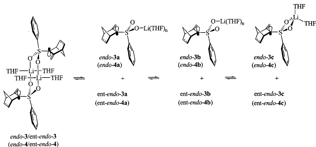
Scheme 3. Monomer-dimer equilibria of the lithioallyl sulfones endo-3 and endo-4
