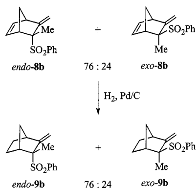
Scheme 7. Stereochemical correlation of the unsaturated sulfones endo - 8b / exo - 8b with the saturated sulfones endo - 9b / exo - 9b
