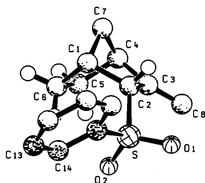
Figure 3. Crystal structure of endo -6
