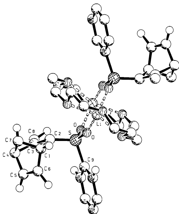
Figure 4. Crystal structure of endo-3/ent-endo-3·2diglyme
