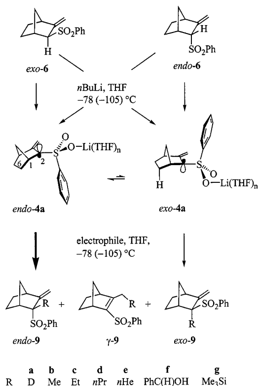
Scheme 6. Reaction of the lithioallyl sulfone 4 with electrophiles
