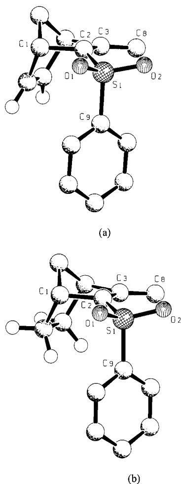
Figure 7. Calculated (HF/6-31+G*) structures of endo-3(-Li + ) (a) and endo-4(-Li + ) (b)
