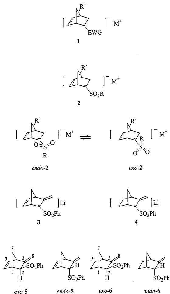
Scheme 1. Sulfonyl-stabilized 2-norbornenyl and 2-norbornyl anions
