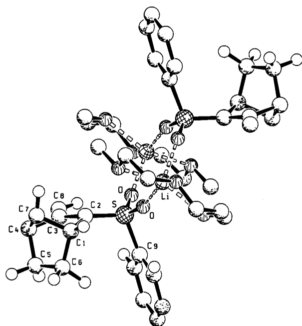
Figure 5. Crystal structure of endo-4/ent-endo-4·2diglyme
