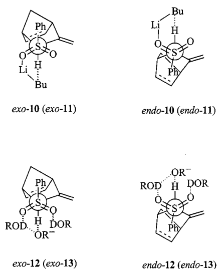
Scheme 9. Transition state models for the base-catalyzed H/D exchange of sulfones exo-5 , endo-5 , and exo-6
