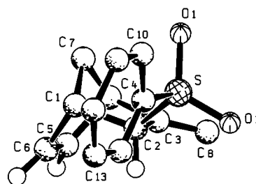
Figure 1. Crystal structure of exo-5
