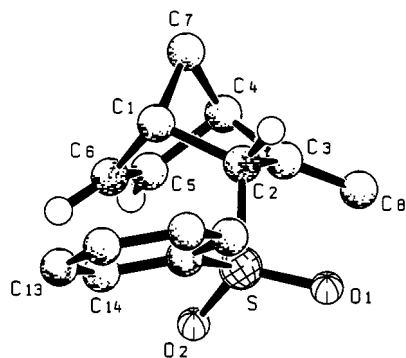
Figure 2. Crystal structure of endo -5
