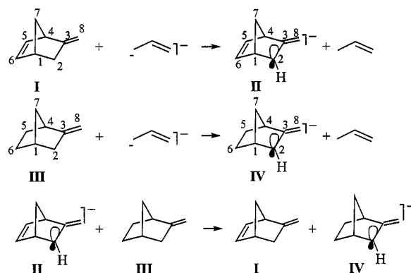
Scheme 2. Isodesmic reactions of methylenenorbornene and methylenenorbornane with the allyl anion
