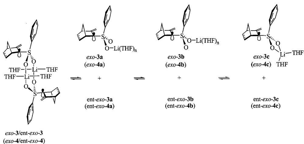
Scheme 4. Monomer-dimer equilibria of the lithioallyl sulfones exo-3 and exo-4
